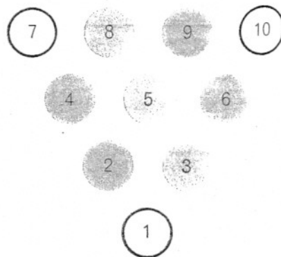
Impossibility proof for Problem 4
